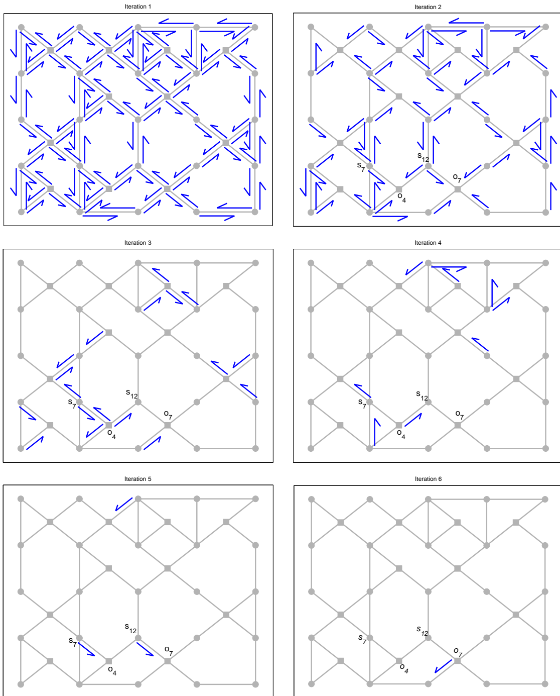
Fig. 10. Information flow dynamics for a data association problem using CSMP. Circle nodes correspond to sensors, and square nodes correspond to targets covered by more than two sensors. The arrows adjacent to edges indicate active communication links and message direction. Sensor s_{12} resumes sending message in iteration five after it was shut off in iteration three. Consequently target node o_7 is waked up in iteration six.
