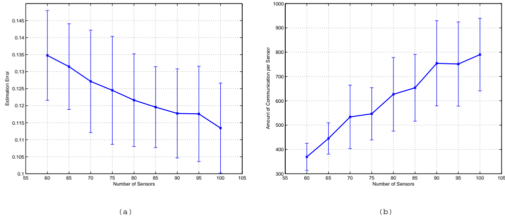
Fig. 11. Error rate and amount of communication for target number estimation using sum-product. The length of the error bar at each data point shows two times of standard deviation.
