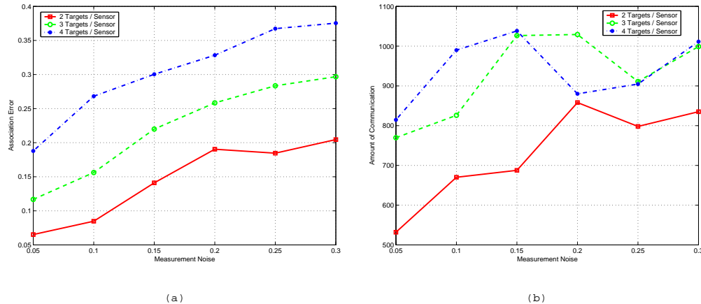
Fig. 8. Data association at various target density and measurement noise levels with TRMP. (a) Association error rate vs. the relative measurement noise variance \omega^2/r^2 . The standard deviation for each point is around 0.075. (b) Amount of communication per sensor vs. the relative measurement noise variance. The standard deviation for each point is around 400.
